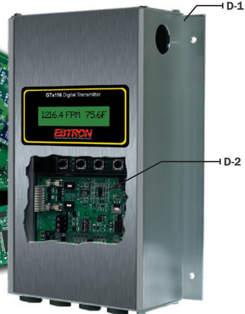
D - EBTRON Digital Transmitter
